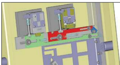
Safe open – Lock on the right unlocked, lock on the left locked, bolts retracted
